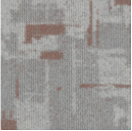
Glitched Gravity B-085
