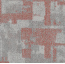
Glitched Gravity C-165
