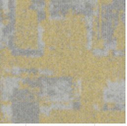
Glitched Gravity D-184
