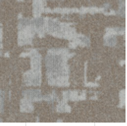
Glitched Gravity D-191
