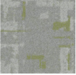
Glitched Gravity B-088
