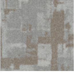
Glitched Gravity C-191
