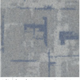
Glitched Gravity B-129
