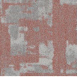
Glitched Gravity D-165
