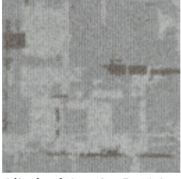
Glitched Gravity B-194
