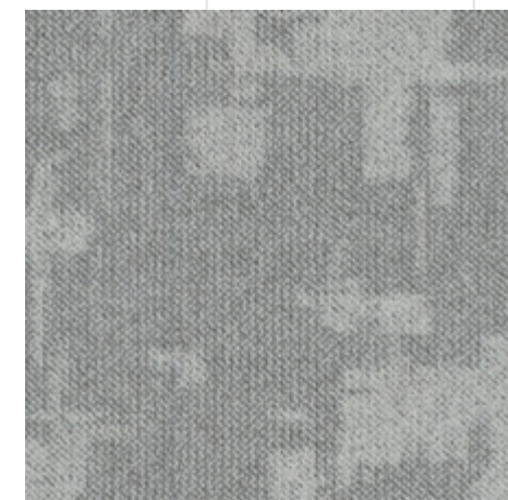
Glitched Gravity A-013
