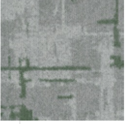
Glitched Gravity B-103
