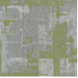
Glitched Gravity C-088
