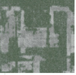
Glitched Gravity D-103
