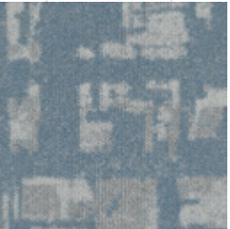
Glitched Gravity D-131
