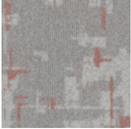
Glitched Gravity B-165
