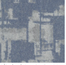
Glitched Gravity D-129
