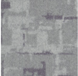
Glitched Gravity B-152
