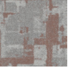
Glitched Gravity C-085
