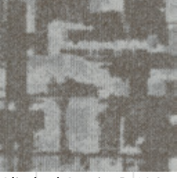
Glitched Gravity D-194
