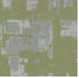
Glitched Gravity D-088
